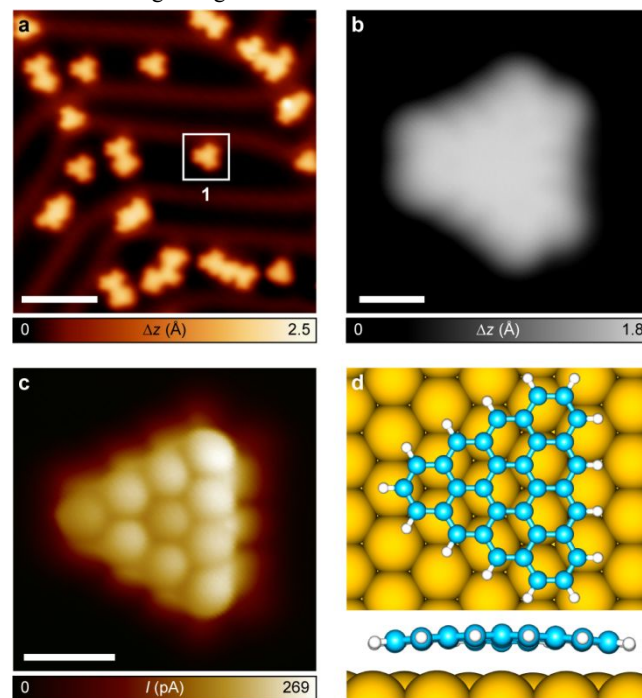
Figure 1. On-surface synthesis and structural characterization of \pi -extended triangulene on Au(111). (a) Overview STM topography image after annealing precursor 2 on Au(111) at 320
