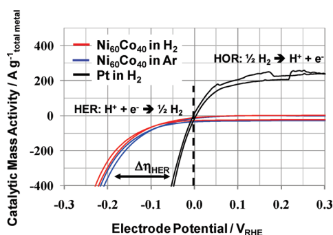
Figure 4. Hydrogen oxidation reaction (HOR) and hydrogen evolution reaction (HER) activity of the \text{Ni}_{60}\text{Co}_{40} bimetallic catalyst in \text{H}_2 -saturated (red) and Ar-saturated (blue) 1 M KOH electrolyte. HER and HOR on a Pt in \text{H}_2 -saturated KOH is shown for comparison (black). \text{Ni}_{60}\text{Co}_{40} shows negligible activity for HOR and a significant HER overpotential \Delta\eta_{\text{HER}} compared to Pt. conditions: 25 °C, scan rate 50 mV/s.
