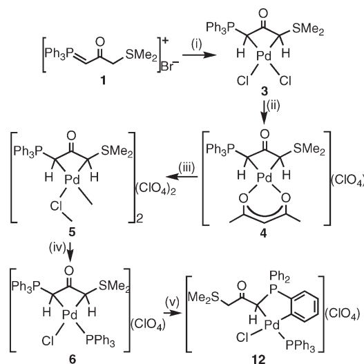
Scheme 2. (i) \text{PdCl}_2(\text{NCMe})_2 , \text{NEt}_3 , \text{MeOH} , -\text{[HNEt}_3\text{]Br} ; (ii) \text{AgClO}_4 , -\text{AgCl} , \text{tlacac} , -\text{TiCl} ; (iii) \text{HCl} , -\text{Hacac} ; (iv) \text{PPh}_3 ; (v) \text{NCMe}/\Delta^a
