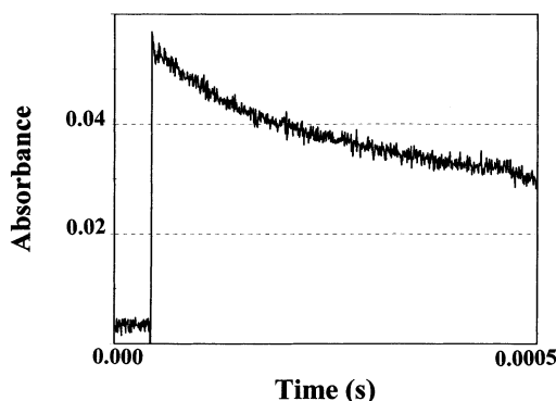
Figure 1. Time-resolved absorption trace at 235 nm after the 193-nm photolysis of a mixture of 1.3 \times 10^{16} molecule \text{cm}^{-3} of \text{C}_2\text{H}_5\text{COC}_2\text{H}_3 in 93 kPa He. The trace is an average of 1000 sweeps.
