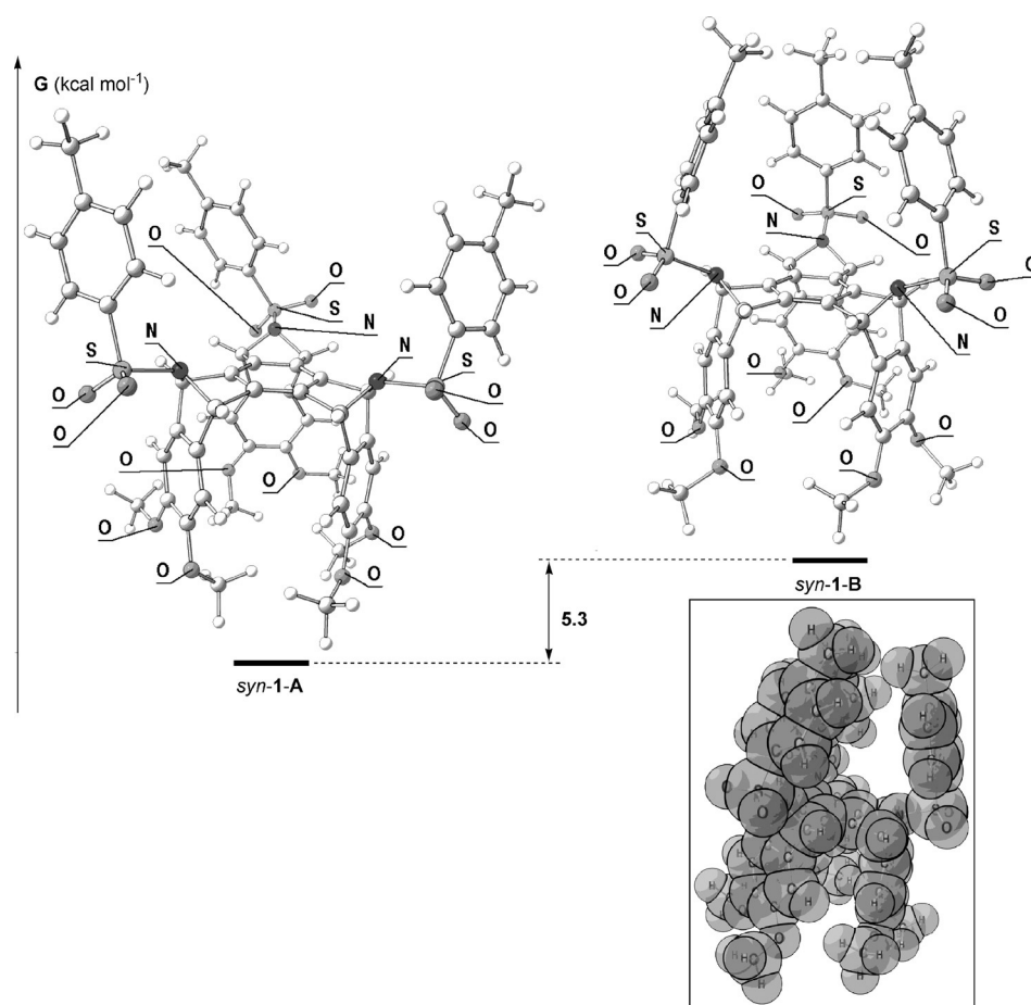
Fig. 2. Syn-1-A and syn-1-B geometries and relative Gibbs energies. Inset: syn-1-B , Van der Waals spheres
