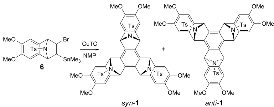
Scheme 3. Cyclotrimerization of vic-Bromostannane 6
