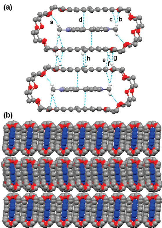
Figure 3. (a) Crystal structure of 1·2 ; the blue lines denote the noncovalent interactions. (b) 2D mosaic-like sheet; the guests are shown in blue. Solvent molecules, PF_6^- counterions, and hydrogen atoms not involved in the interactions were omitted for clarity.
