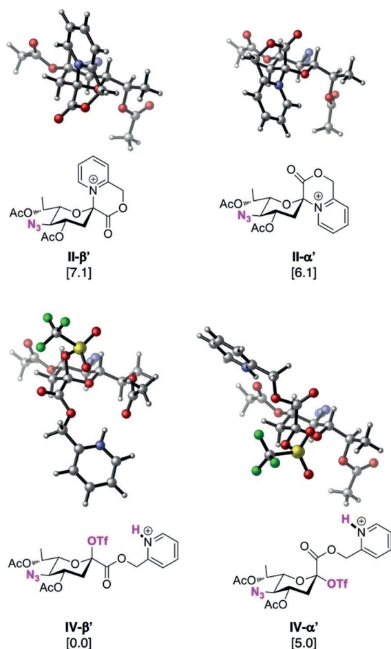
Figure 2. Computed geometries of simplified relevant reactive intermediates for the glycosylation reaction with donor 2 . Entries are calculated at SMD (CH 2 Cl 2 )-M06-2X/6-311 + G(d,p). The corresponding solvated Gibbs free energy in kcal mol -1 at T = 253.15 K is denoted in brackets. In the Figure the HOTf is omitted for II-α' and II-β' for clarity reasons.
