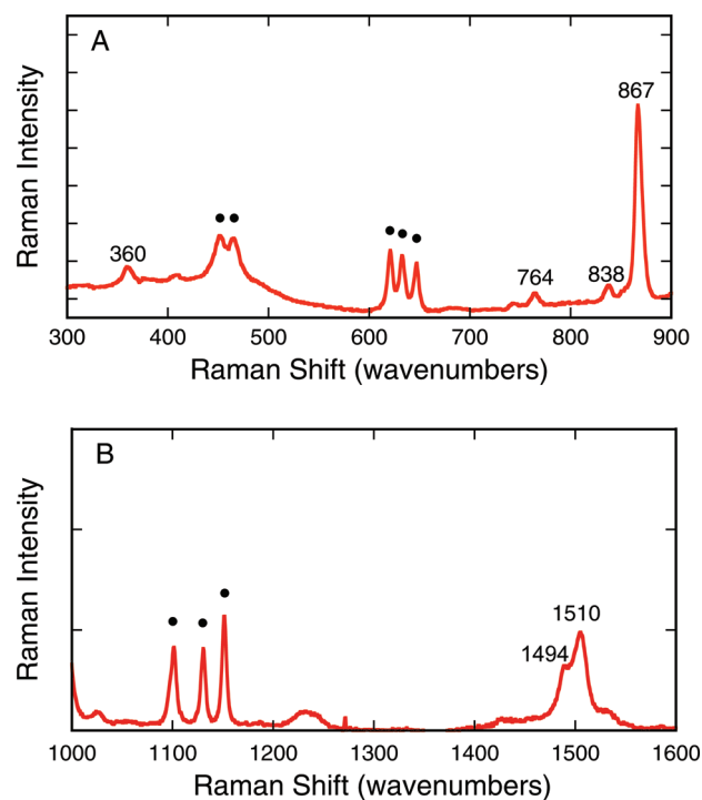
Figure 10. Low frequency (A) and high frequency (B) resonance Raman spectra of 6 using 458 nm excitation. Raman bands for the Na_2SO_4 internal standard are indicated with black dots. Vibrational assignments are given in Table 4.
