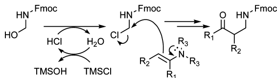
Scheme 1. Proposed Mechanism
