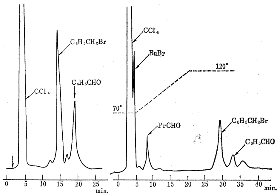
Fig. 1c. Reaction Products from Benzyl Ether with I in Carbon Tetrachloride
