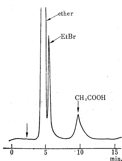
Fig. 1a. Reaction Products from Ethyl Ether with I in Ethyl Ether
