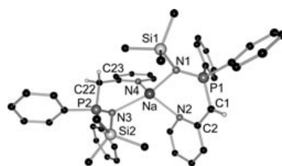
Figure 4. Solid-state structure of 4 ; for clarity reasons only the hydrogen atoms at the bridging carbon atoms are depicted.
