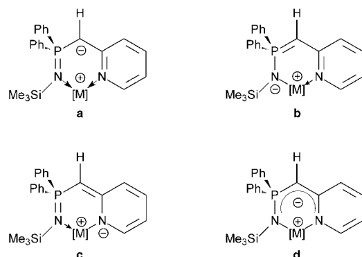
Scheme 3. Resonance forms of [M\{Ph_2P(CHPy)\}(NSiMe_3)]^- : a indicates a carbanionic ylidic contribution, b shows the amidic ylenic resonance structure, c emphasises the amidic olefinic resonance form and d visualises the delocalisation of the negative charge.
