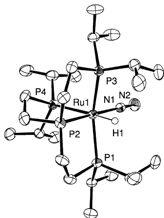
Figure 6. ORTEP diagram (50% thermal ellipsoids, selected hydrogen atoms only) of the complex cation of [\text{Ru}(\text{N}_2)\text{H}(\text{PPi}_3)][\text{BF}_4] \cdot \text{THF} ( 7 · [\text{BF}_4] ).
