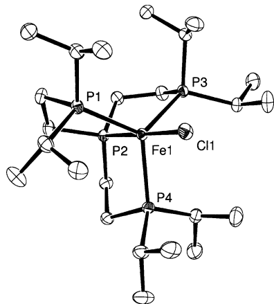
Figure 1. Oak Ridge Thermal Ellipsoid Plot (ORTEP) diagram (50% thermal ellipsoids, non-hydrogen atoms) of the complex cation of [\text{FeCl}(\text{PPi}_3)][\text{BPh}_4] ( 2 · [\text{BPh}_4] ).
