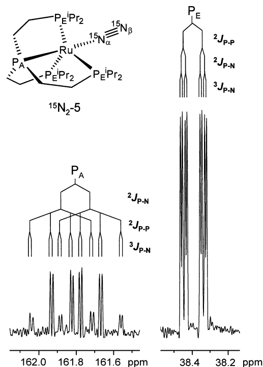
Figure 3. Resolution-enhanced ^{31}\text{P}\{^1\text{H}\} NMR spectrum (202 MHz, benzene- d_6 ) of \text{Ru}(^{15}\text{N}_2)(\text{PPi}_3) ( ^{15}\text{N}_2 - 5 ).
