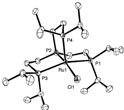
Figure 2. ORTEP diagram (50% thermal ellipsoids, non-hydrogen atoms) of one of the two complex cations of [\text{RuCl}(\text{PPi}_3)][\text{BPh}_4] , ( 3 · BPh 4 ), within each asymmetric unit.
