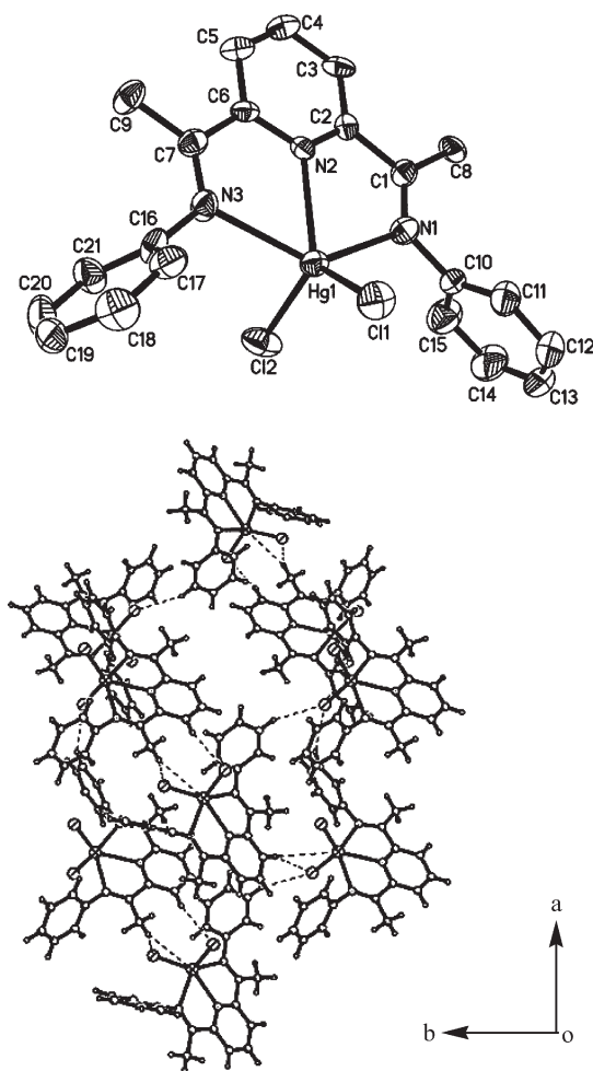
Figure 1. Top: Molecular structure of complex 1 (the other molecule and CH 3 CN molecules have been omitted for clarity). Bottom: Packing diagram of complex 1 along the c axis. Hydrogen bonds are indicated by dashed lines.
