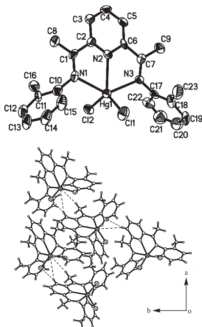
Figure 4. Top: Molecular structure of complex 4 (the other molecule and \text{CH}_3\text{CN} molecules have been omitted for clarity). Bottom: Packing diagram of complex 4 along the c axis. Hydrogen bonds are indicated by dashed lines.
