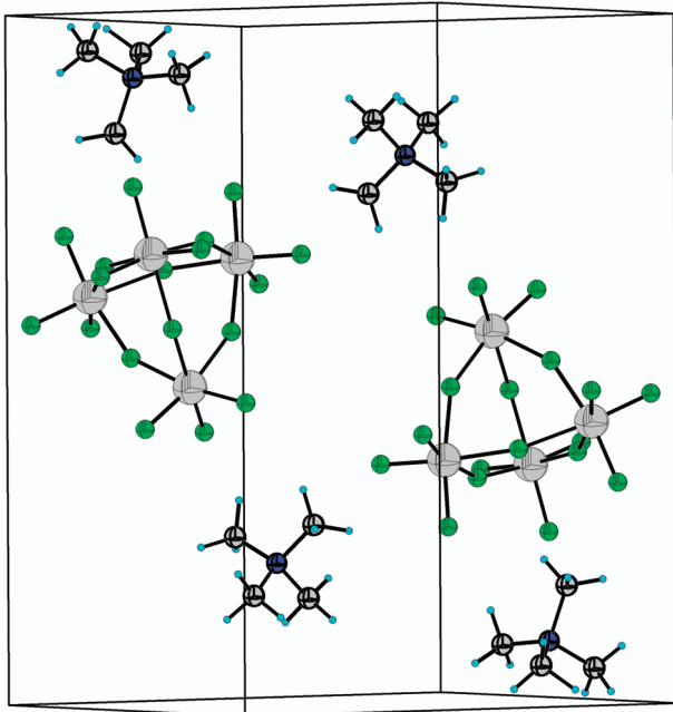
Figure 1. Part of the crystal structure of [\text{Me}_4\text{N}]_2[\text{Ti}_4\text{F}_{18}] .
