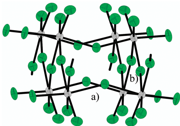
Figure 5. \text{Ti}-\text{F}_b-\text{Ti} angles in the crystal structure of [\text{H}_3\text{O}][\text{Ti}_2\text{F}_9] [(a) 143.7(2)^\circ ; (b) 166.4(2)^\circ ] and \text{CsTi}_2\text{F}_9 [(a) 149.3(6)^\circ ; (b) 156.3(4)^\circ ].
