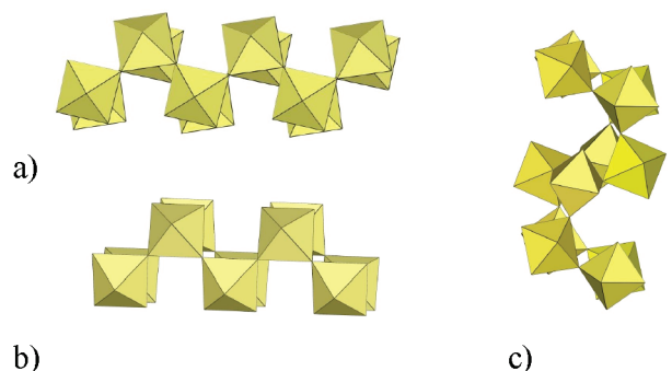
Figure 6. Formation of infinite [\text{Ti}_2\text{F}_9]_n double chains in the crystal structures of \text{CsTi}_2\text{F}_9 (a), [\text{H}_3\text{O}][\text{Ti}_2\text{F}_9] (b), and \text{O}_2\text{Mn}_2\text{F}_9 (c). 18
