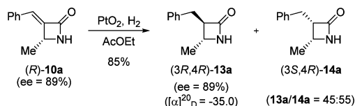
Scheme 4. Determination of Absolute Configuration of \alpha -Alkylidene- \beta -amino Esters
