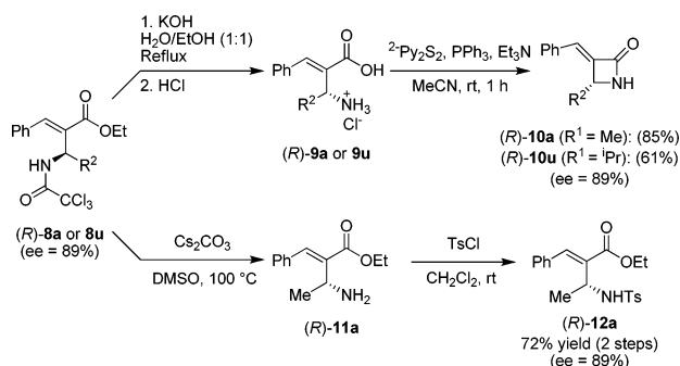
Scheme 3. Application of \alpha -Alkylidene- \beta -amino Esters to Synthesis of Optically Active \beta -Lactams
