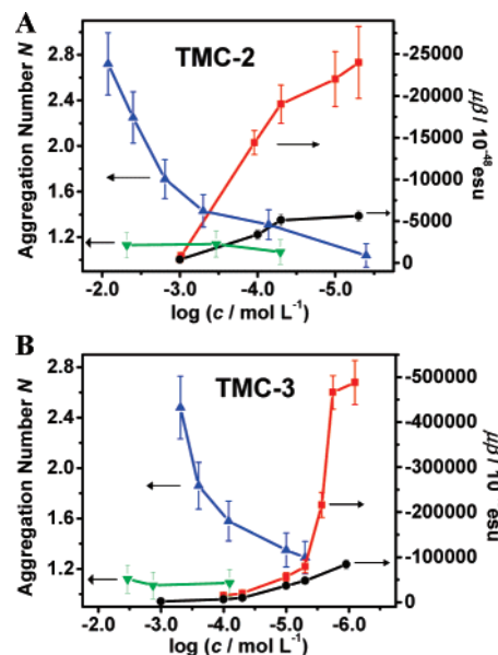
Figure 8. Comparative PGSE NMR-derived aggregation number ( N , left scale) data and EFISH-derived \mu\beta data (right scale) as a function of concentration for twisted chromophores TMC-2 (A) and TMC-3 (B). PGSE NMR data are obtained from CD 2 Cl 2 ( \blacktriangle ) and DMSO- d 6 ( \blacktriangledown ) solutions. EFISH measurements are performed in CH 2 Cl 2 ( \blacksquare ) and DMF ( \bullet ) solutions. Lines are drawn as guides to the eye. c = concentration.
