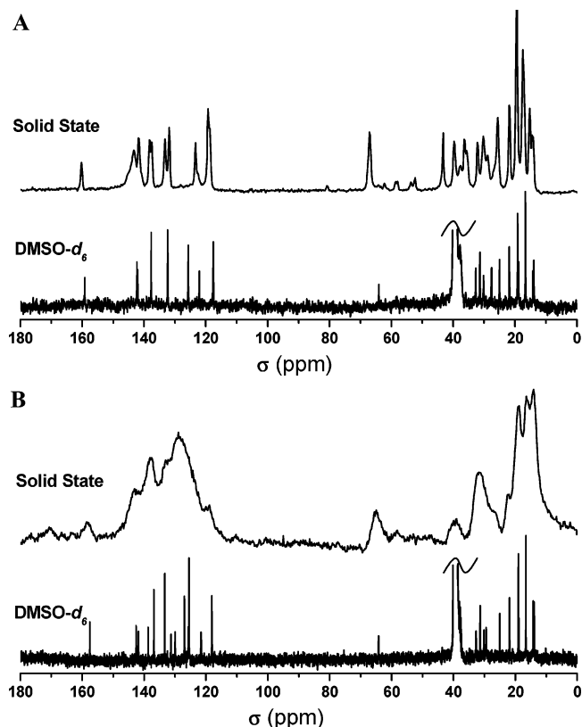
Figure 6. (A) 13 C NMR spectra of chromophore TMC-2 in the solid state (top) and DMSO- d 6 solution (bottom). (B) 13 C NMR spectra of chromophore TMC-3 in the solid state (top) and DMSO- d 6 solution (bottom).
