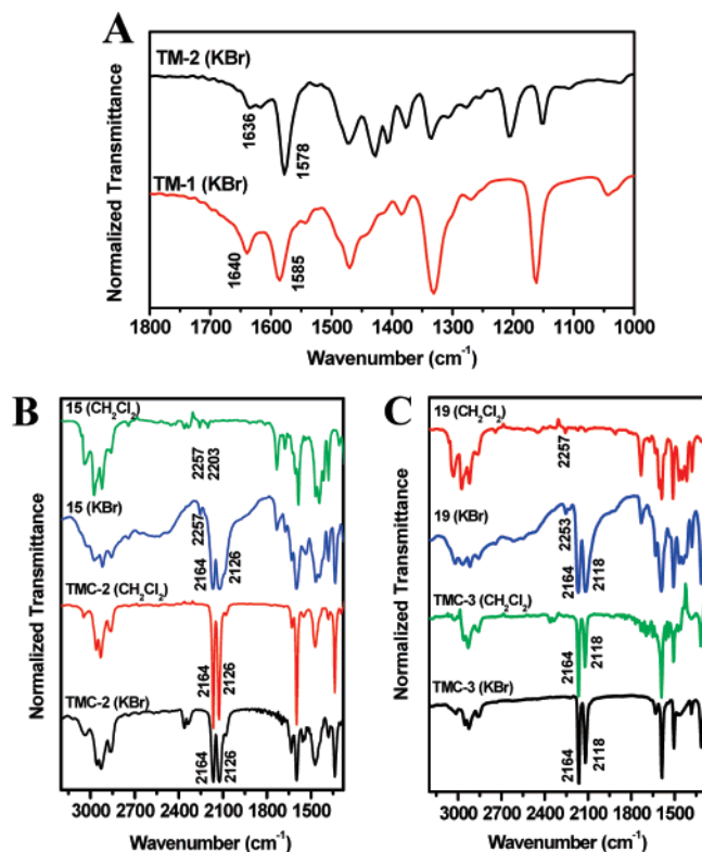
Figure 5. (A) IR spectra of chromophores TM-1 and TM-2 as KBr pellets. (B) IR spectra of TMC-2 and its neutral precursor 15 in a KBr pellet and CH 2 Cl 2 solution. (C) IR spectra of TMC-3 and its neutral precursor 19 in a KBr pellet and CH 2 Cl 2 solution.
