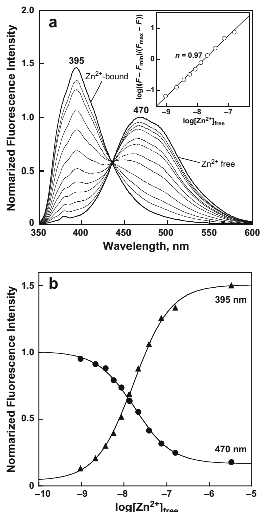
Figure 2. (a) Emission spectra of ZID-1 (1 \mu M) excited at 335 nm in \text{Zn}^{2+} /NTA buffered system (50 mM HEPES, pH 7.20, 0.1 M \text{KNO}_3 ; 10 mM NTA, 0–9.5 mM \text{ZnSO}_4 ) and in 50 mM HEPES buffer (pH 7.20) containing 4 \mu M \text{ZnSO}_4 . Inset: Hill plot at 470 nm. The Hill coefficient ( n ) was determined from the slope. (b) Plots of fluorescence intensities at 395 nm (triangles) and 470 nm (circles) with best-fit curves for the dissociation constant of 17.1 \times 10^{-9} M.
