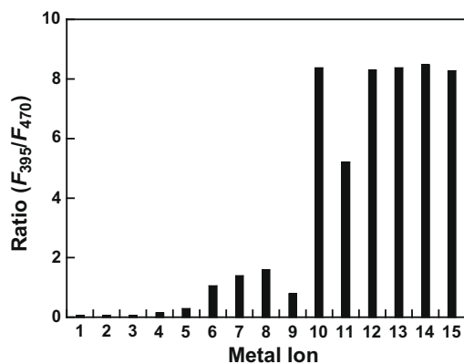
Figure 3. Fluorescence ratio of ZID-1 (1 \mu M) between 395 nm and 470 nm as a function of various added metal cations (5 mM for \text{Na}^+ , \text{K}^+ , \text{Ca}^{2+} , and \text{Mg}^{2+} , 10 \mu M for all other cations) in 50 mM HEPES (pH 7.20, 0.1 M \text{KNO}_3 ). 1: no metal; 2: \text{Na}^+ ; 3: \text{K}^+ ; 4: \text{Mg}^{2+} ; 5: \text{Ca}^{2+} ; 6: \text{Fe}^{2+} ; 7: \text{Co}^{2+} ; 8: \text{Ni}^{2+} ; 9: \text{Cu}^{2+} ; 10: \text{Zn}^{2+} ; 11: \text{Cd}^{2+} ; 12: \text{Zn}^{2+} + \text{Na}^+ ; 13: \text{Zn}^{2+} + \text{K}^+ ; 14: \text{Zn}^{2+} + \text{Mg}^{2+} ; 15: \text{Zn}^{2+} + \text{Ca}^{2+} .
