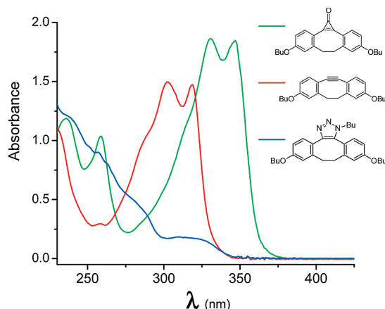
Figure 1. Spectra of 5 \times 10^{-5} M methanol solutions of cyclopropenone 2c (green), acetylene 3c (red), and triazole 4c (blue) ( R = Bu ).
