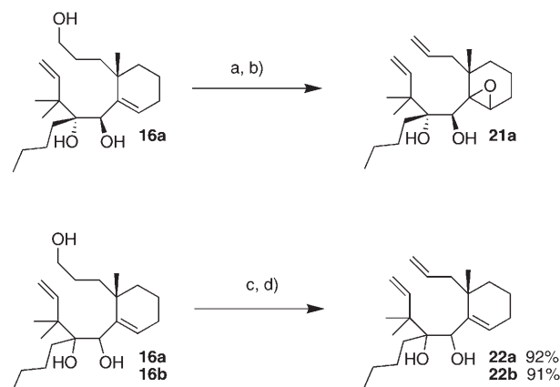
Scheme 8. Synthesis of metathesis precursors 22a and 22b : a) \text{PBu}_3 , o -nitrophenylselenocyanate, THF, 20 °C; b) \text{H}_2\text{O}_2 , THF, 20 °C, 20%; c) \text{PBu}_3 , o -nitrophenylselenocyanate, THF, 20 °C; d) \text{H}_2\text{O}_2 , (\text{NH}_4)_6\text{Mo}_7\text{O}_{24} \cdot 4\text{H}_2\text{O} , THF, -10 °C.
