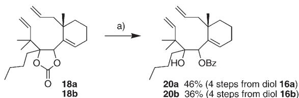
Scheme 7. Synthesis of metathesis precursors 20a and 20b : a) \text{PhLi} , THF, -78 °C.
