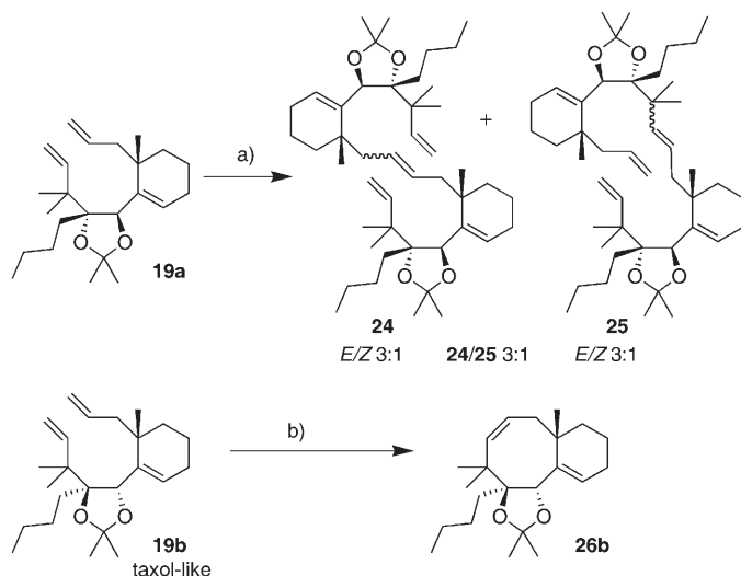
Scheme 9. Metathesis of acetonides 19a and 19b : a) 5 mol % Grubbs 2, CH 2 Cl 2 , reflux, 87 % for the mixture of 24 and 25 ; b) 5 mol % Grubbs 2, 1,2-dichloroethane, reflux, quant.
