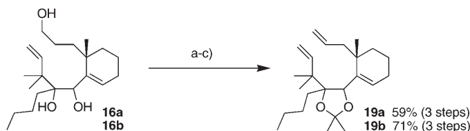
Scheme 6. Synthesis of metathesis precursors, acetonides 19a and 19b : a) 2,2-Dimethoxypropane, CSA, 20 °C; b) \text{PBu}_3 , o -nitrophenylselenocyanate, THF, 20 °C; c) \text{H}_2\text{O}_2 , THF, 20 °C. CSA = camphor-10-sulfonic acid.
