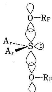
Fig. 1. Molecular Orbital Representation of a Sulfurane
