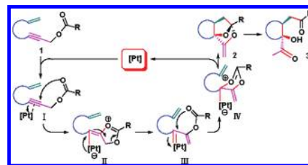
Scheme 3. PtCl 2 -Catalyzed [3 + 2] Cycloaddition of Enynes and the Proposed Mechanism
