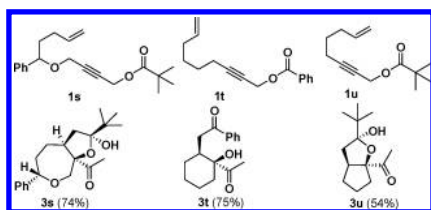
Scheme 2. Modified Pt-Catalyzed Reaction of Enynyl Esters
