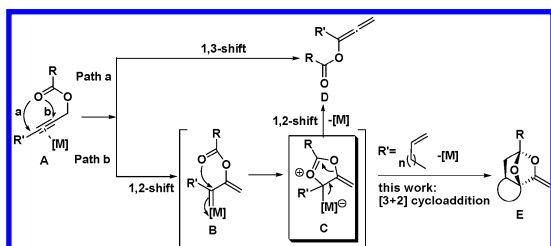
Scheme 1. Transition-Metal-Catalyzed Reactivity of Propargylic Carboxylates
