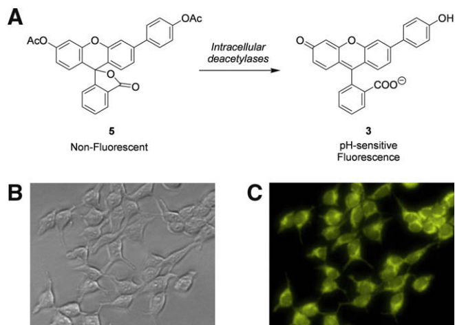
Figure 4. (A) Intracellular deacetylation of compound 5 to give anthofluorescein 3 . HeLa cells were incubated for 2 h with a 25 \mu\text{M} solution of diacetylated anthofluorescein 5 . (B) Brightfield. (C) Fluorescent image with 488 nm excitation and no emission filter.
