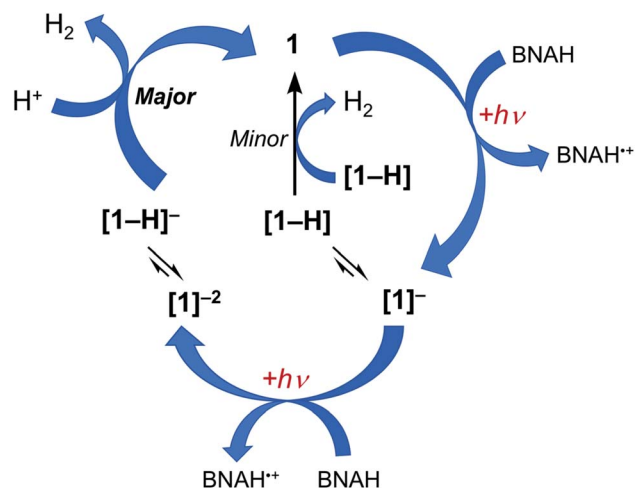
Fig. 6 Proposed catalytic cycle of photocatalytic H_2 production by 1 , showing two possible pathways, one through the reaction of two molecules [1\text{-H}] (minor pathway) and the other through the protonation of [1\text{-H}]^- .
