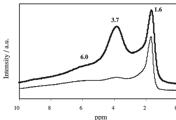
Figure 3. ^1\text{H} MAS NMR spectra of parent HMCM-22 (bold line) and dealuminated HMCM-22 (narrow line), respectively.
