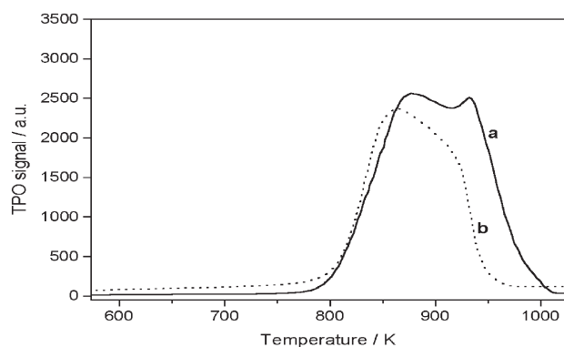
Figure 2. TPO profiles of coked 6% Mo/HMCM-22 (a) and 6% Mo/HMCM-22-D (b) after reaction at 1023 K for 24 h. (TPO experiments were carried out using 30 mg of catalyst at a 10% \text{O}_2/\text{He} flow rate of 15 \text{ ml min}^{-1} and temperature raising rate of 10 \text{ K min}^{-1} .)
