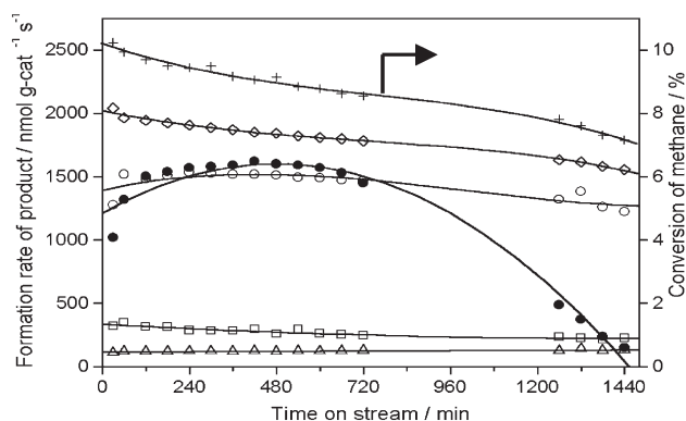
Figure 1. Catalytic performance of 6% Mo/HMC-22-D catalyst at 1023 K, 0.3 MPa and 2700 \text{ml g}^{-1} \text{h}^{-1} versus time on stream; +, \circ , \square , \triangle , and \diamond represent methane conversion, formation rates of benzene, naphthalene, \text{C}_2 hydrocarbons, and hydrogen ( \times 1/2 ), separately. Solid circle ( \bullet ) represents formation rate of benzene on 6% Mo/HMC-22 catalyst under same reaction conditions.
