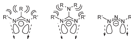
Chart 3. Effect of Sterics on N -Orbital Projection in Amidinate, Guanidinate, and Triazenide Ligands
