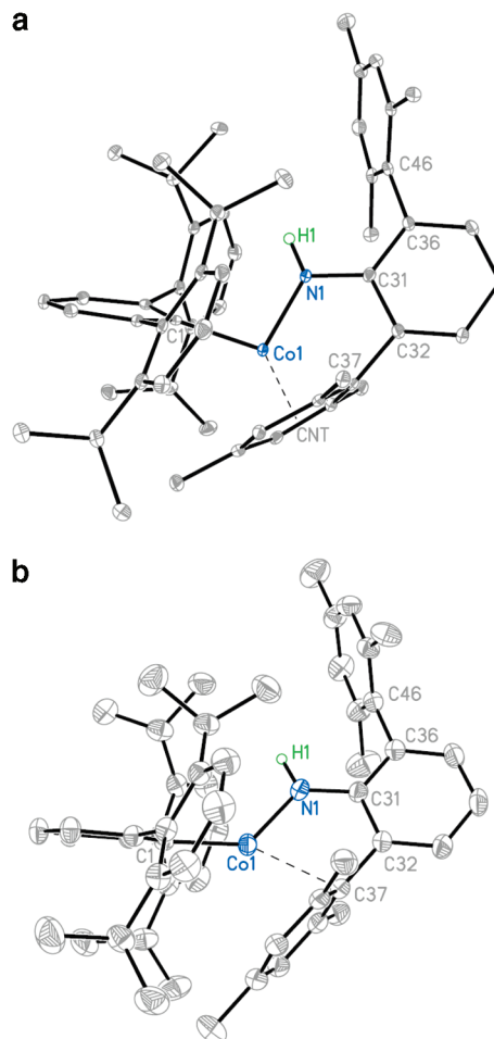
Figure 3. (a) Molecular structure of 3a at 90 K with thermal ellipsoids presented at a 30% probability level. Hydrogen (except N–H) atoms are not shown for clarity. (b) Molecular structure of 3b at 240 K with thermal ellipsoids presented at a 30% probability level. Hydrogen (except N–H) atoms are not shown for clarity.
