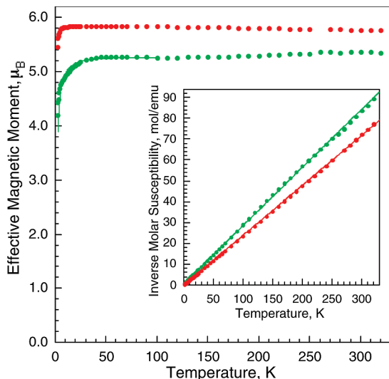
Figure 4. Temperature dependence of the effective magnetic moment of 1 , red, and 2 , green. The parameters for the fit of 2 shown between 2 and 100 K are S = 2 , g = 2.15 , and D = 6 \text{ cm}^{-1} . Inset: the inverse molar magnetic susceptibility of 1 and 2 and their corresponding Curie–Weiss law fits.
