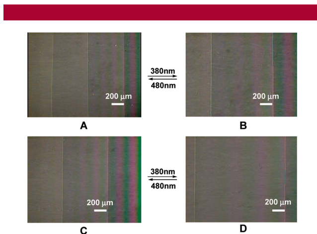
Figure 4. Polarized optical micrographs (40× magnification) of (A) 0.1 wt % ( P )- E,E - 1 and (C) 0.1 wt % of ( M )- E,E - 1 dissolved in E7 at 25 °C in a wedge cell (A and C, before irradiation; B and D, after irradiation at 380 nm for 15 min).
