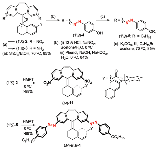
Scheme 1. Synthesis of ( M )- 11 and ( M )- E , E - 1
