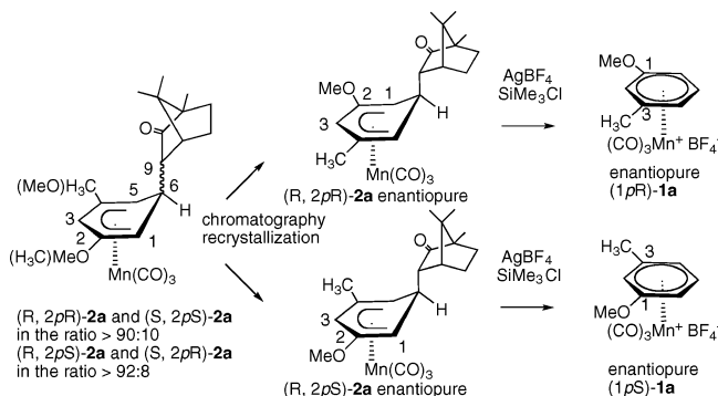
Scheme 2. Separation of the Diastereoisomers 2a and Rearomatization
