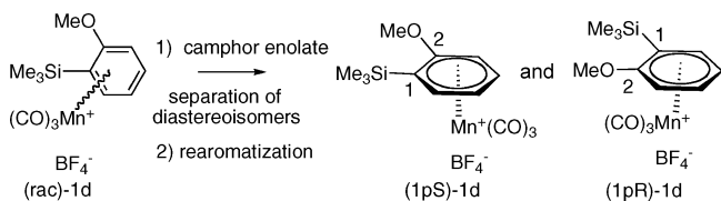
Scheme 3. Resolution of o -Trimethylsilylanisole Complex ( rac )- 1d
