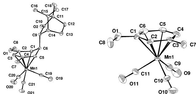
Figure 1. ORTEP views of complexes ( R ,2 pR )- 2a and ( 1pR )- 1a .
