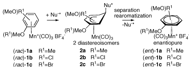
Scheme 1. Resolution of ( \eta^6 -Arene)Mn(CO) 3 + Complexes Using a Chiral Nucleophile “Round Trip”
