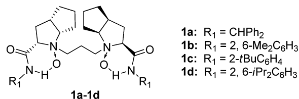
Figure 1. N,N' -Dioxide ligands evaluated.
