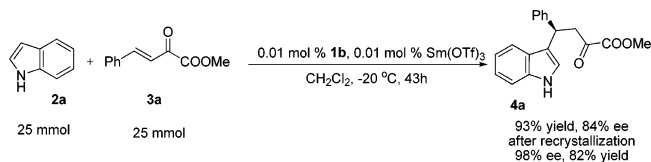
Scheme 1. Scaled-up Version of Friedel–Crafts Alkylation of Indole 2a with \beta,\gamma -Unsaturated \alpha -Ketoester 3a
