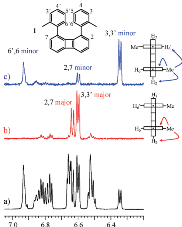
FIGURE 3. Trace a: aromatic region (600 MHz at -118^{\circ}\text{C} in \text{CD}_2\text{Cl}_2 ) displaying ^1\text{H} signals for the major and minor conformers of 1 . Trace b: NOE due to irradiation of the major methyl signal (1.87 ppm), showing significant enhancement for two aromatic signals of the major conformer (syn). Trace c: NOE due to irradiation of the minor methyl signal (1.59 ppm), showing significant enhancements for three aromatic signals of the minor conformer (anti).
