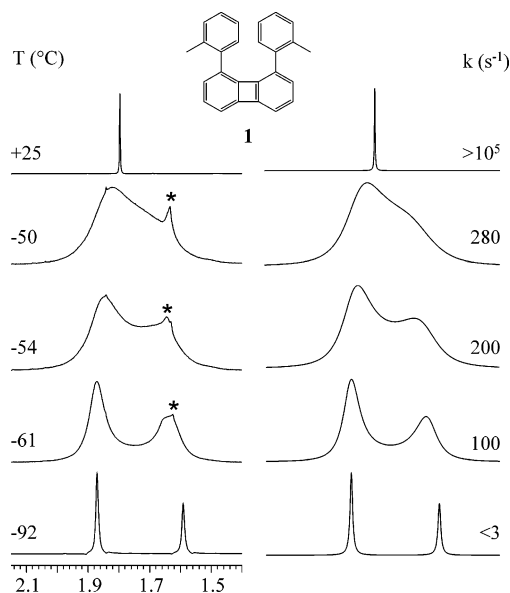
FIGURE 2. Left: experimental NMR 1 H signal (600 MHz in CD 2 Cl 2 ) of the methyl group of 1 as function of temperature (the starred line is a trace of HDO present in the solvent). Right: line shape simulation obtained with the rate constants indicated.
