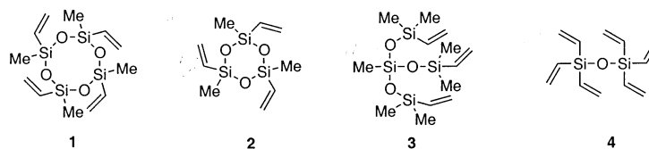
Fig. 1. Structures of 1,3,5,7-tetramethyl-1,3,5,7-tetravinylcyclotetrasiloxane ( D_4^Y , 1 ), 1,3,5-trimethyl-1,3,5-trivinylcyclotrisiloxane ( D_3^Y , 2 ), tri(vinyltrimethylsiloxy)-methylsilane ( 3 ) and hexavinylidisiloxane ( 4 ).
