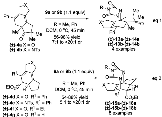
Scheme 3. Cycloadditions of Cyclohexadienes 4a,b,d–g with TADs 9a and 9b a
