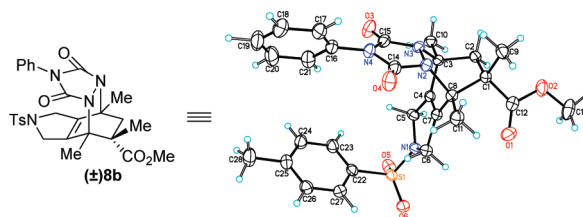
Figure 1. ORTEP diagram of cycloadduct (±)- 8b .
