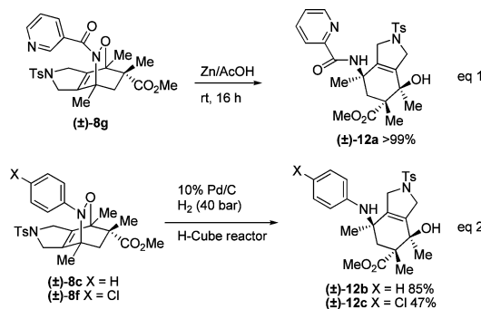
Scheme 2. N–O Bond Cleavage of Nitroso Cycloadducts
