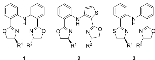
Figure 1. Bis(oxazoline) ligands.
