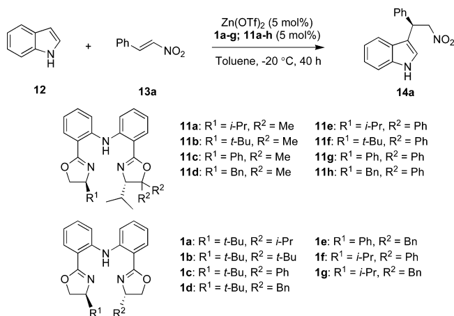
Scheme 3. Asymmetric Friedel–Crafts Alkylation of Indole (12) with trans - \beta -Nitrostyrene (13a) Using Ligands 1a–g and 11a–h
