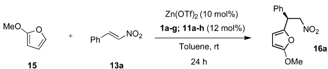
Scheme 4. Asymmetric Friedel–Crafts Alkylation of 2-Methoxyfuran (15) with trans - \beta -Nitrostyrene (13a) Using Ligands 1a–g and 11a–h
