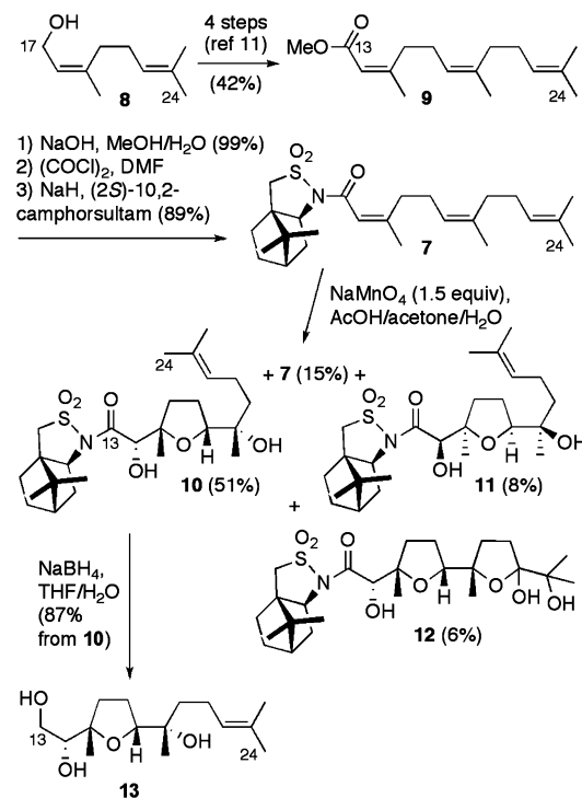
Scheme 2. Synthesis of the C13–C24 Portion of Eurylene
