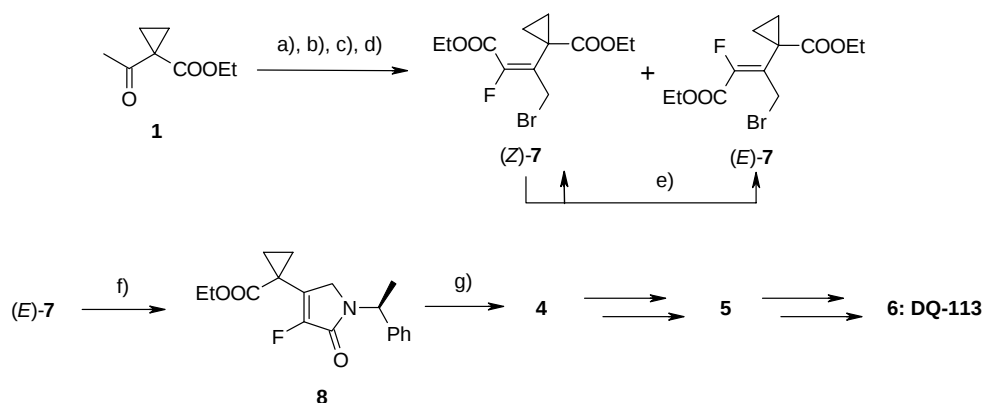
Scheme 2. Improved synthesis of DQ-113 (the Reformatsky reaction/isomerization strategy): a) BrFCHCO 2 Et (1.0 eq.), Zn (3.0 eq.), cat. I 2 / benzene, reflux, 2 h; b) SOCl 2 (1.2 eq.) / pyridine, -10°C, 3 h; c) DBU (1.1 eq.) / CH 2 Cl 2 , rt, 17 h; d) NBS (1.0 eq.), cat. AIBN / CHCl 3 , reflux, 16 h; e) cat. NBS, cat. AIBN / benzene, reflux, 16 h; f) ( S )-1-phenylethylamine (1.1 eq.), NaHCO 3 (2.5 eq.) / EtOH, reflux, 3 h; g) H 2 (5 kg/cm 2 ), Raney Ni / EtOH, rt, 3.5 h; total yield: 2.1% (14 steps).
