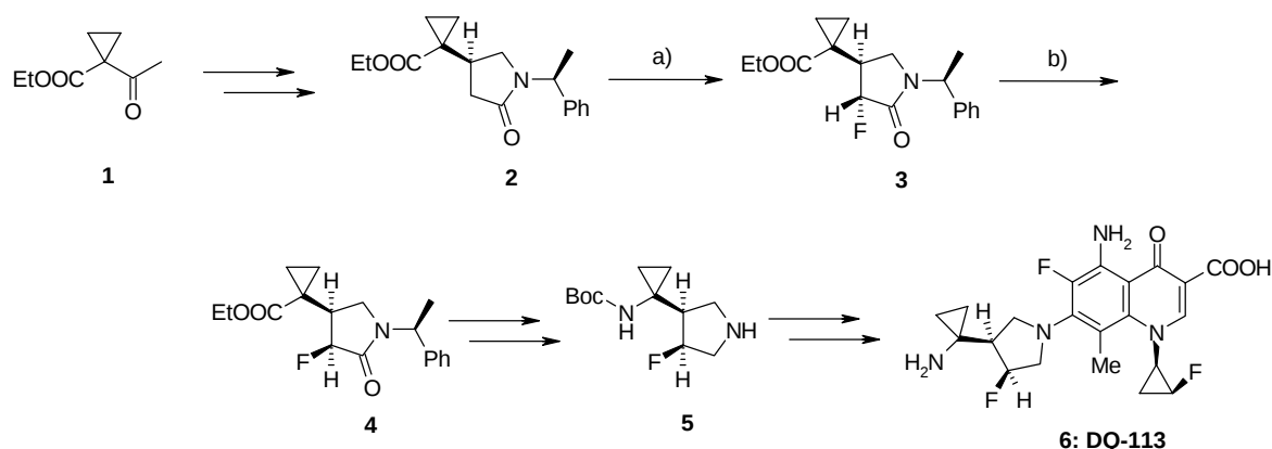
Scheme 1. Preparative synthesis of DQ-113 (fluorination/isomerization strategy): a) LDA (1.3 eq.), (PhSO 2 ) 2 NF (1.6 eq.) / THF, -78°C, 2 h, then rt, 20 min; b) LDA (1.1 eq.), 2,6-di- tert -butylphenol (1.2 eq.) / THF, -78°C, 10 min, then rt, 1 h; total yield: 0.6% (16 steps).
