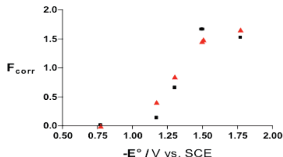
Figure 4. Experimental (red \blacktriangle ) and calculated (black \blacksquare ) product ratios \text{F}_{\text{corr}} as a function of mediator potential for the indirect electrolyses of 2-BF 4 .
