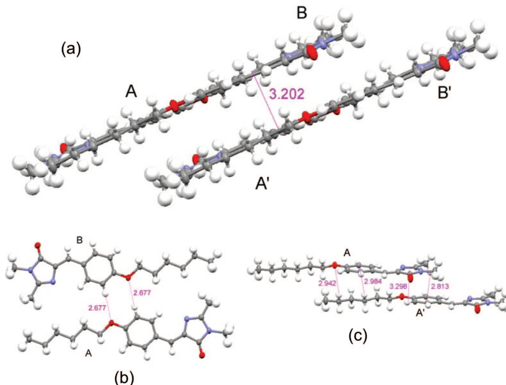
Figure 9. (a) Tetramer unit of HexOBDI taken from the X-ray structure. (b,c) Dimer units showing the AB and AA' interactions.
