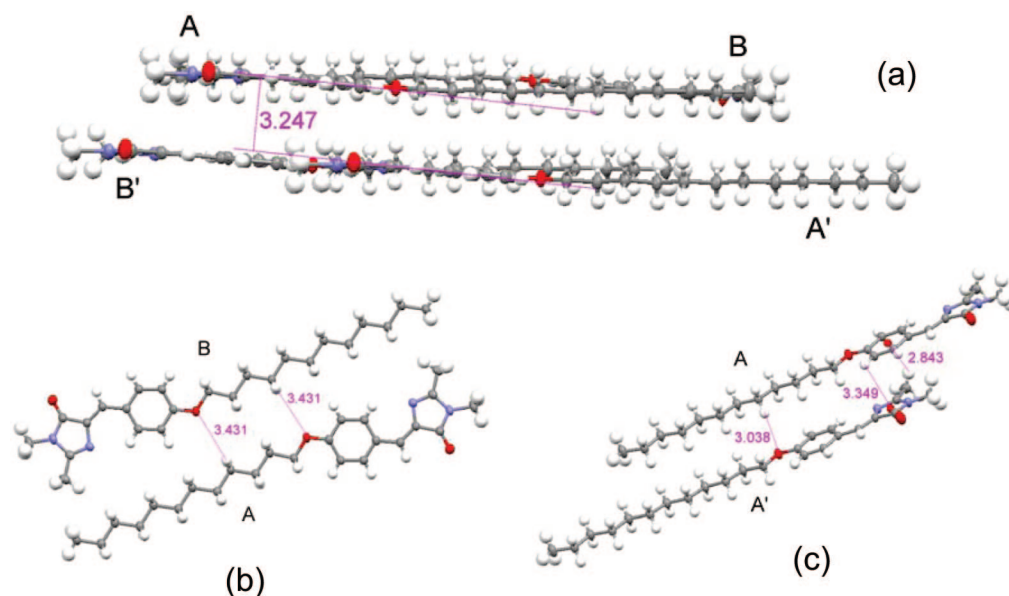
Figure 10. (a) Tetramer unit of DdecOBDI taken from the X-ray structure. (b,c) Dimer units showing the AB and AA' interaction.
