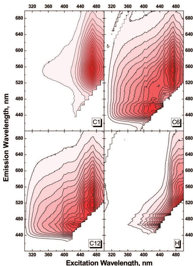
Figure 3. Excitation–emission contour plots of solid ROBBDI samples. The difference between the neighboring lines corresponds to the constant intensity difference on a linear scale. Deeper colors correspond to higher intensities.
