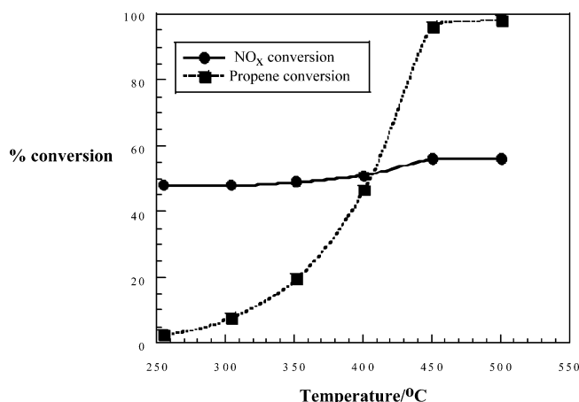
Figure 8. \text{NO}_x reduction/propene oxidation on 20 \text{ m}^2/\text{g} of \text{Ce}_{0.7}\text{Zr}_{0.3}\text{O}_2 as a function of temperature. Propene oxidizes ( >90\% to \text{CO}_2 ) \text{NO}_x reduces to \text{N}_2 ( >99\% ) selectively. 65,66
