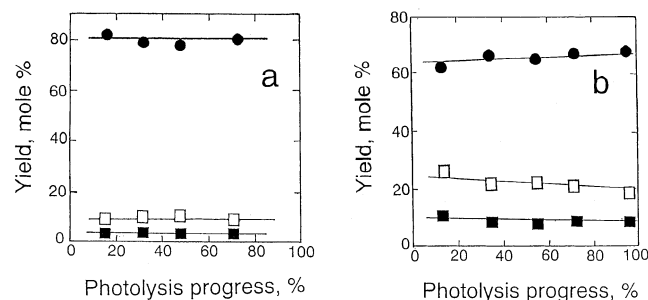
Fig. 3. Hydrocarbon product yield (in relative mole percent) at different stages of (a) (C_2H_5)_2Se photolysis with fluence 127 \text{ mJ cm}^{-2} and (b) of (C_2H_5)_2Te photolysis with fluence 100 \text{ mJ cm}^{-2} . n -C 4 H 10 (□); C 2 H 6 (■); C 2 H 4 (●).
