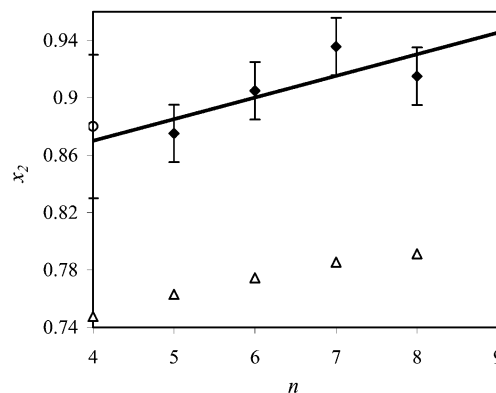
Figure 5. Relationship between x_{2(\text{UCST})} and the number of carbons in R n for [R n mim][PF 6 ] (1) + butan-1-ol (2): ◆, experiment; ○, 1-butyl estimated from experimental data; △, COSMOtherm.
