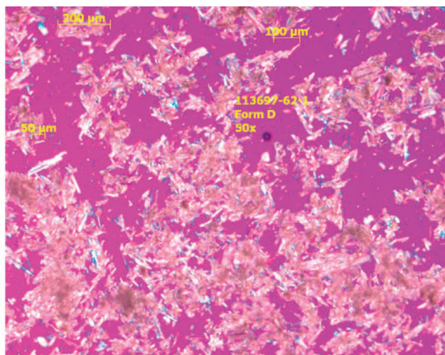
Figure 6. Photomicrographs of slow (left) and fast (right) filtering solids (both images are at 50× magnification).
