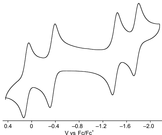
Figure 4. Cyclic voltammogram of 2a (V vs Fc/Fc + , in 0.1 M n Bu 4 NClO 4 /CH 2 Cl 2 , scan rate 100 mV/s, room temperature).
