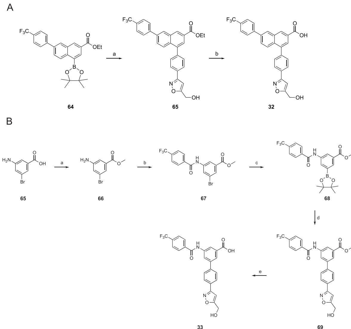
Scheme 4. (A) Synthesis of Naphthalene-Containing Isoxazole Derivative 32 a
