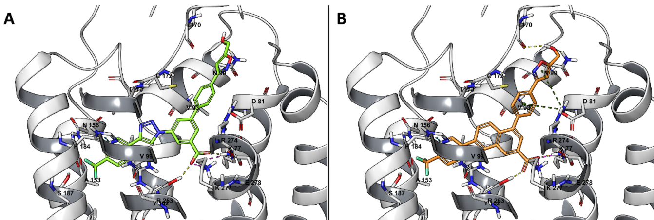
Figure 1. Docking pose of compound 29 (A), in green, and compound 32 (B), in orange, at the P2Y 14 R structure (gray), obtained by MD-refined homology modeling using an agonist-bound P2Y 12 R structure (PDB ID: 4PXZ 34 ) as the template.
