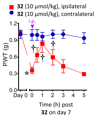
Figure 3. Reversal of CCI-induced mechano-allodynia in the mouse induced by compound 32 (10 \mu\text{mol kg}^{-1} , i.p.). Mean \pm SD is shown, n = 3 ; ANOVA, * P < 0.05 vs day 0 and ^{\dagger}P < 0.05 vs day 7 post-injury. 32 was dissolved in 5% DMSO in water as a vehicle, and a volume of 0.2 mL was injected.
