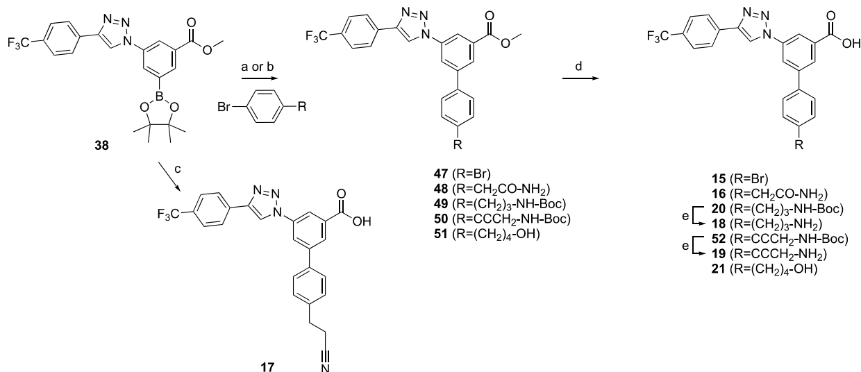
Scheme 2. Synthesis of Triazole-Containing Derivatives with Acyclic Replacement of the Piperidine Ring of 3a a
