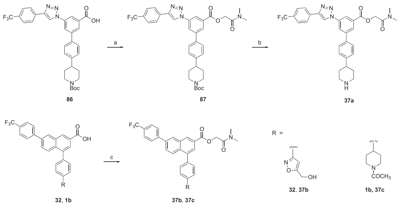
Scheme 6. Synthesis of Prodrug Derivatives 37a–37c a
