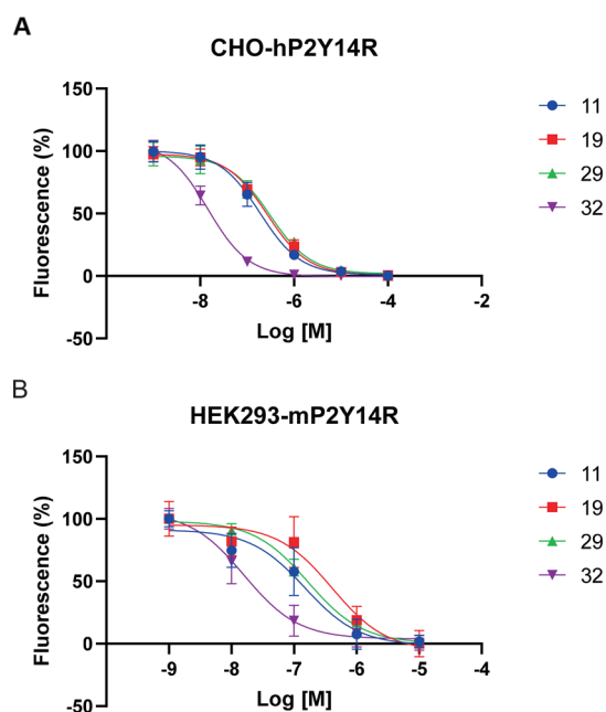
Figure 2. Inhibition of binding of fluorescent antagonist 2 at hP2Y 14 R (A) and at mP2Y 14 R (B) by four novel P2Y 14 R antagonist analogues (mean \pm SD, n = 3 –4 independent determinations, performed in triplicate).
