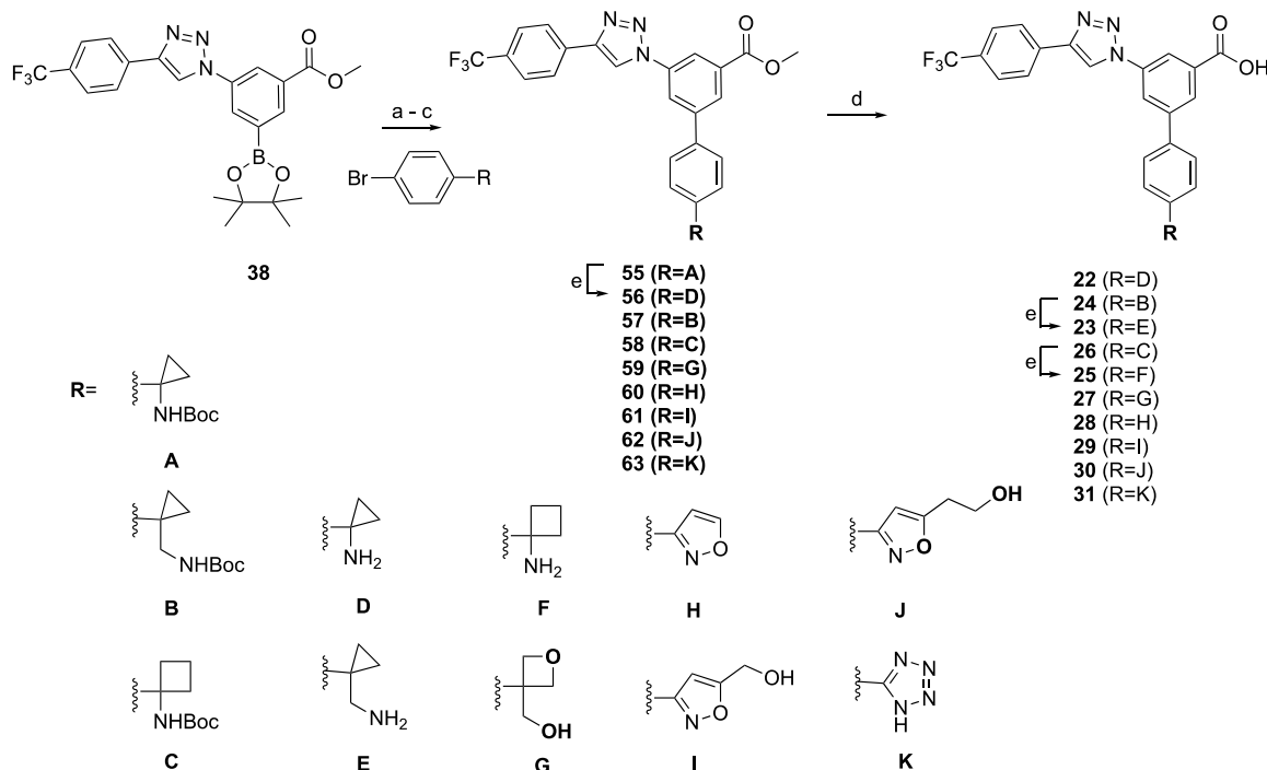
Scheme 3. Synthesis of Triazole-Containing Derivatives with Cyclic Replacement of the Piperidine Ring of 3a a
