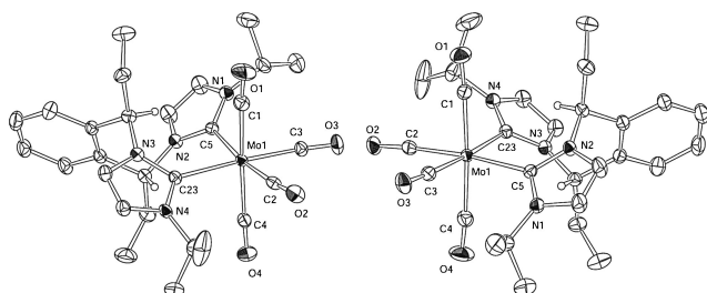
Figure 2. ORTEP drawings of ( R,R )- 5a (left) and ( S,S )- 5a (right). All hydrogen atoms except on benzylic carbons are omitted for clarity.
