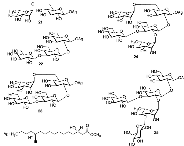
Fig. 4. Structures of the Products ( 21 – 25 ) Obtained by Partial Methanolysis of 14
