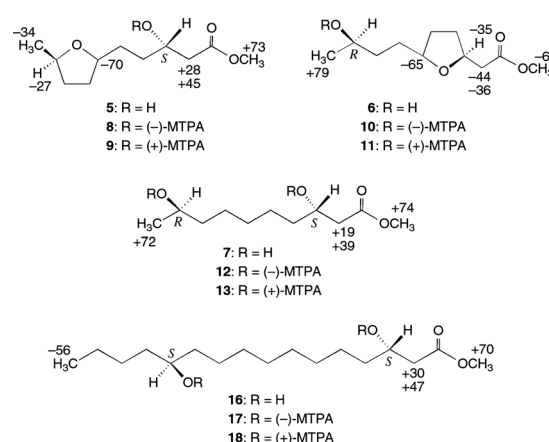
Fig. 2. Structures of 5 — 13 and 16 — 18 , and Values of ^1\text{H} -NMR Chemical Shift Difference (ppm) [ \Delta\delta : \delta(-)\text{-MTPA} — \delta(+)\text{-MTPA} Ester ( \times 10^{-3} )] for MTPA Esters (in \text{CDCl}_3 , 600 MHz)
