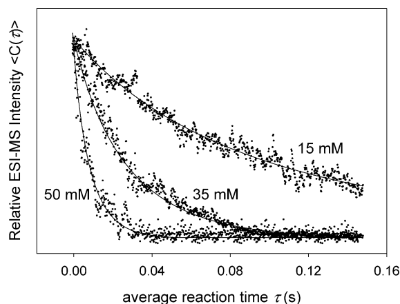
Figure 4. Demetalation kinetics of chlorophyll a ( m/z 894) in methanol recorded by ESI-MS at three different concentrations of HCl. Solid line represent fits based on eq 5, with C(t) = a \exp(-k_{\text{obs}}t) .
