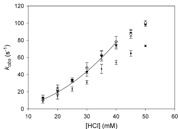
Figure 5. Pseudo-first-order rate constants k_{\text{obs}} for the demetalation of chlorophyll a as a function of HCl concentration. Solid triangles are the results of ESI-MS kinetics that were analyzed based on eq 5, taking into account laminar flow effects. The solid line is a quadratic fit to these data ( k_{\text{obs}} values measured for the two highest acid concentrations were not considered for the fit). Open circles are data measured by standard optical stopped-flow spectroscopy. Also shown are k_{\text{obs}} values that were obtained from the ESI-MS data by using a “plug-flow” data analysis that fails to take into account laminar flow effects (small solid squares). Error bars are standard deviations, based on at least four independent measurements for each acid concentration.
