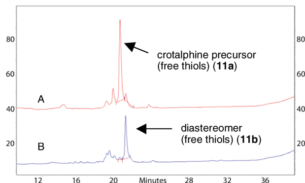
Figure 3. Reverse-phase HPLC analyses of crude crotalphine precursor 11 (free thiols). (A) Crude crotalphine precursor (free thiols) from cyclic ortho ester resin 5a . (B) Crude diastereomer (free thiols) from cyclic ortho ester resin 5b . (For details, see Supporting Information.)
