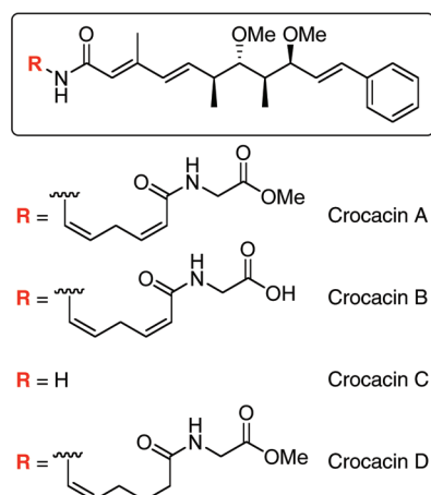
FIGURE 1. Structure of crocacin A–D.
