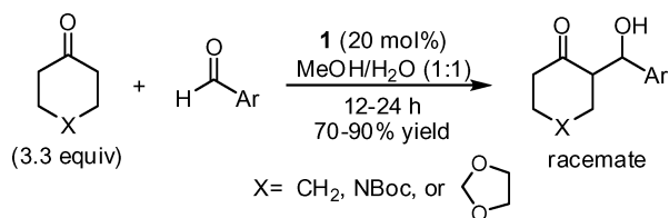
Scheme 1 2-Picolyamine ( 1 ) catalyzed racemic aldol product formation.
