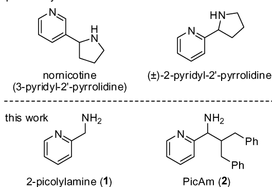
Fig. 1 Pyridine based aldol organocatalysts.
