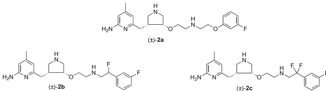
Figure 1. Chemical structures of 2a–c.
