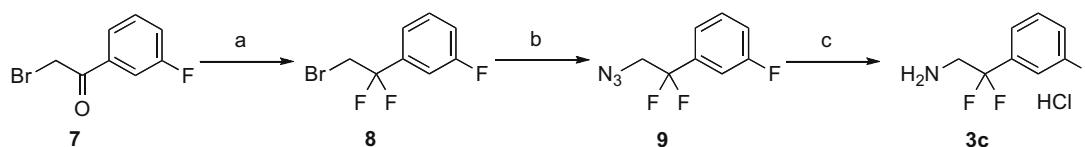
Scheme 2. Reagents and conditions: (a) DAST (neat), rt, 7 days, 70%; (b) NaN_3 , DMSO, 110 °C, 1 h, 88%; (c) Pd(OH)_2/C , H_2 , EtOH/1 N HCl (2:1), rt, 24 h, 91%.
