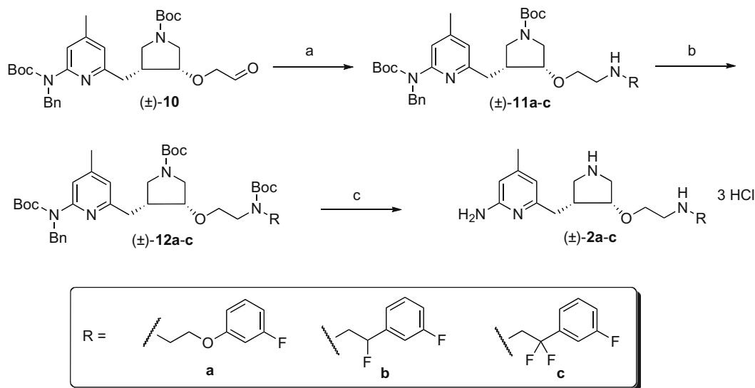
Scheme 3. Reagents and conditions: (a) (i) 3a–c , THF, rt, 5 min; (ii) NaBH(OAc) 3 , rt, 3 h; (b) (Boc) 2 O, Et 3 N, MeOH, rt, 12 h, 48–60% for two steps; (c) Pd(OH) 2 /C, H 2 , 2:1 EtOH/HCl (12 N), rt, 500 psi, 40 h, 85–91%.
