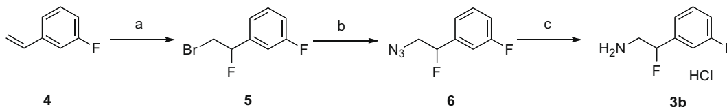
Scheme 1. Reagents and conditions: (a) NBS, Et_3N \cdot 3HF , CH_2Cl_2 , 0 °C to rt, 12 h, 85%; (b) NaN_3 , DMSO, 65 °C, 4 h, 85%; (c) Pd(OH)_2/C , H_2 , EtOH/1 N HCl (2:1), rt, 24 h, 98%.
